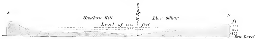
Section 1 mile further west.
